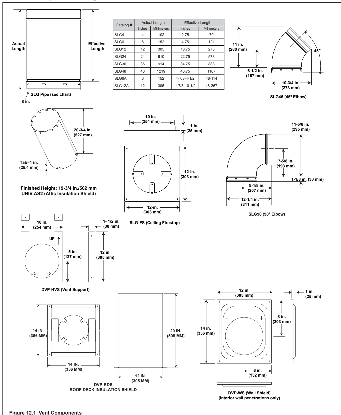
Figure 12.1 Vent Components
