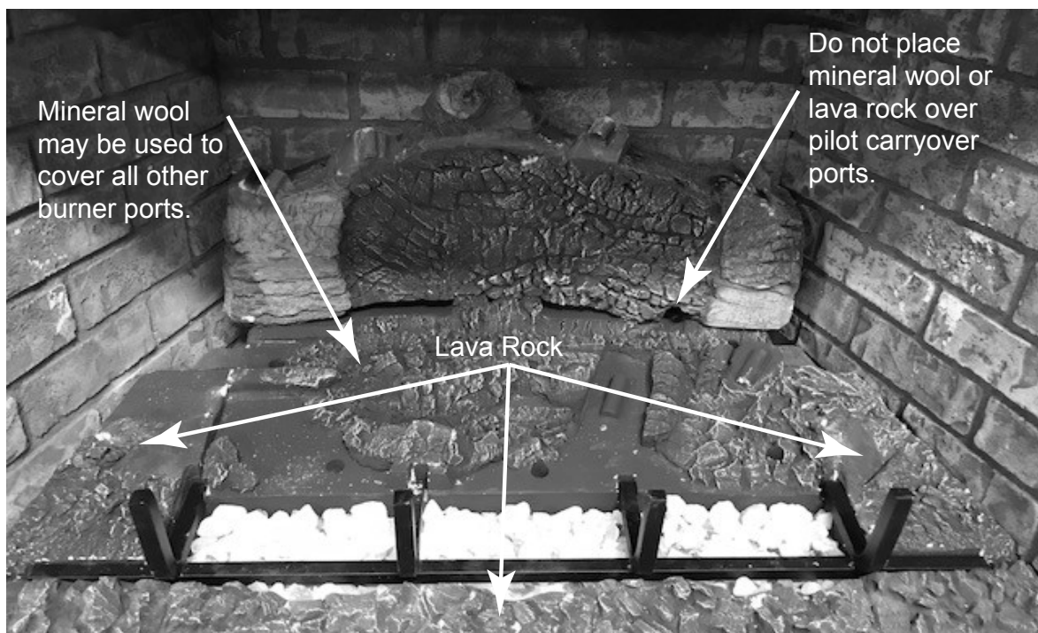
Figure 11.22 Placement of Mineral Wool and Lava Rock
