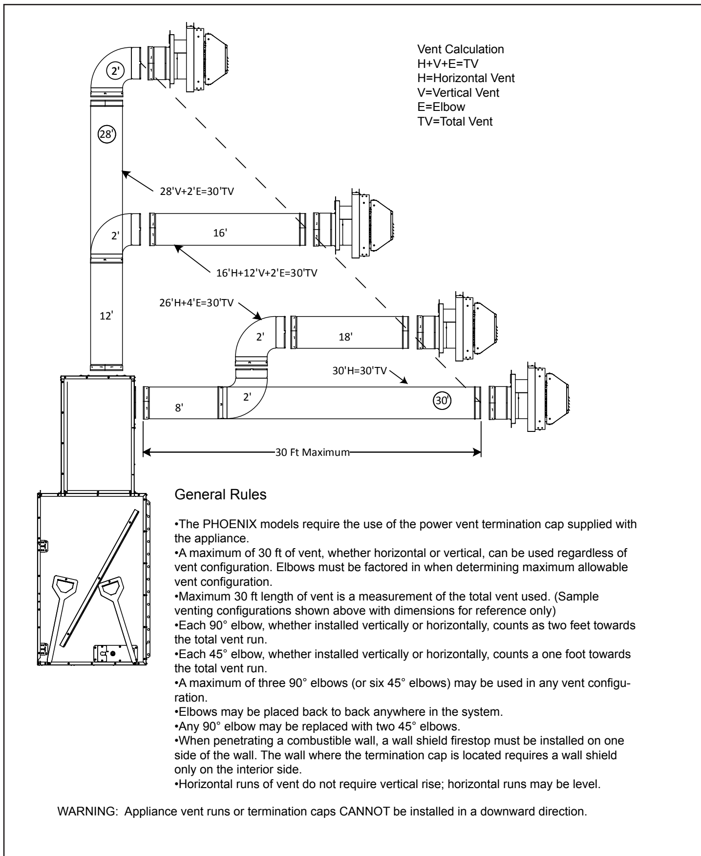
Figure 4.5 Venting
