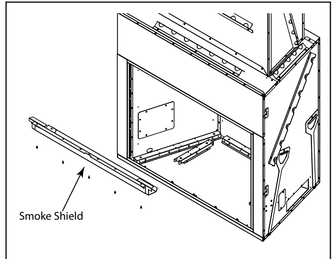
Figure 11.4 Smoke Shield
