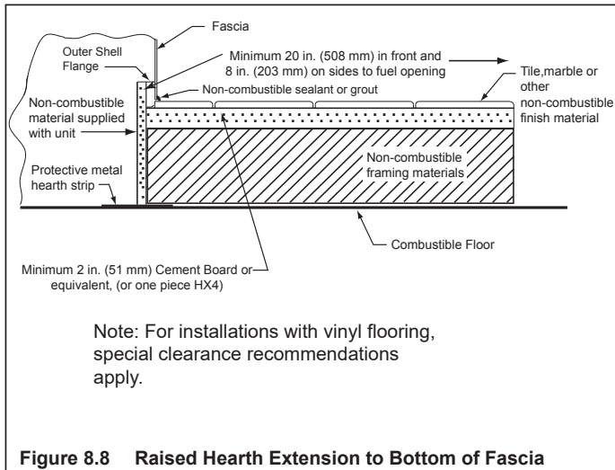
Figure 8.8 Raised Hearth Extension to Bottom of Fascia
