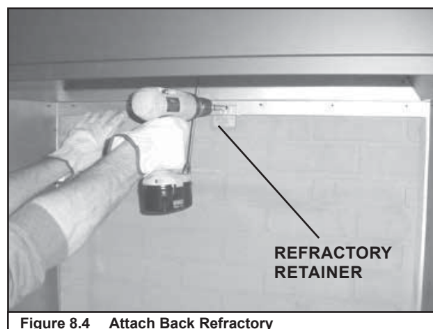
Figure 8.4 Attach Back Refractory
