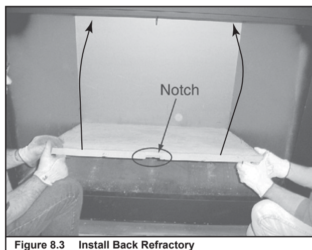
Figure 8.3 Install Back Refractory
