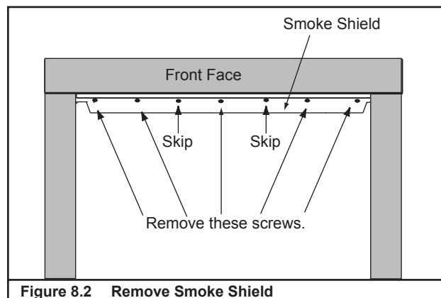
Figure 8.2 Remove Smoke Shield
