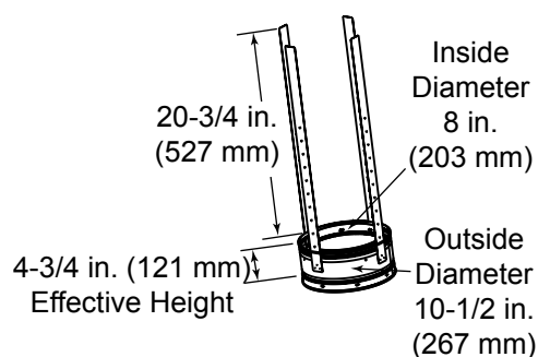
SL3 Chimney Stabilizer
