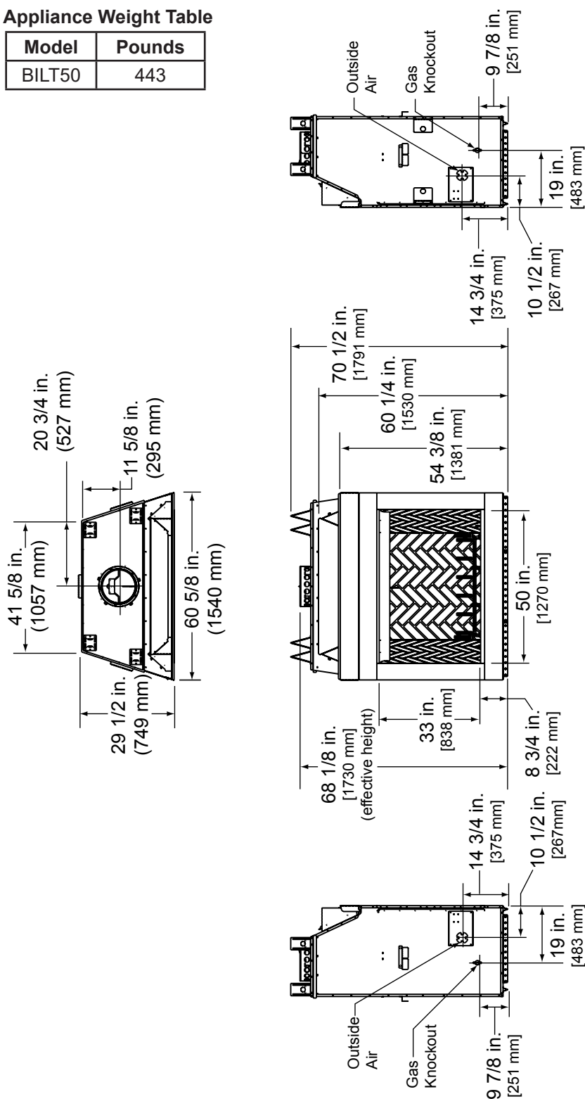
Figure 3.1 Appliance Dimensions
