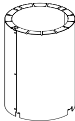
Assembled Diameter: 17 in./432 mm Height: 24 in./610 mm AS10 Straight Attic Insulation Shield
