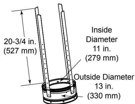
SL11 Chimney Stabilizer
