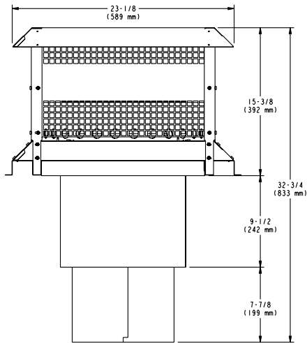
ST1175 - Square Termination Cap
