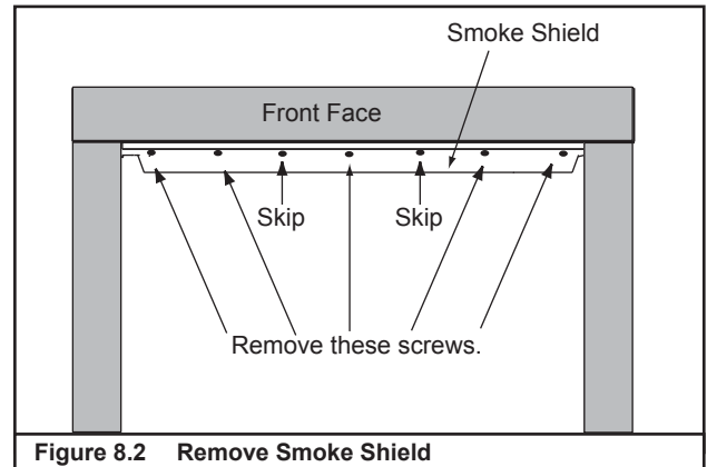
Figure 8.2 Remove Smoke Shield
