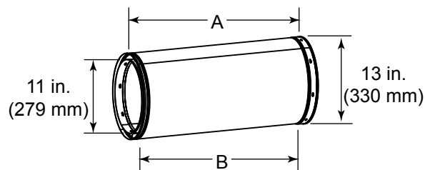
Chimney Sections
