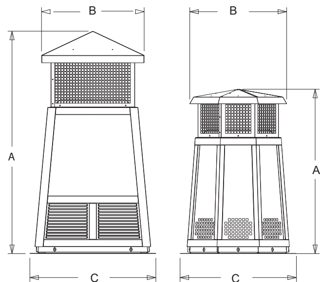
DTS134/146-BK/CP DTO134/146-BK/CP Decorative Caps
