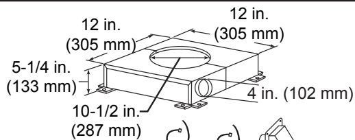
CAK4A Chimney Air Kit
