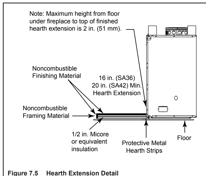
Figure 7.5 Hearth Extension Detail
