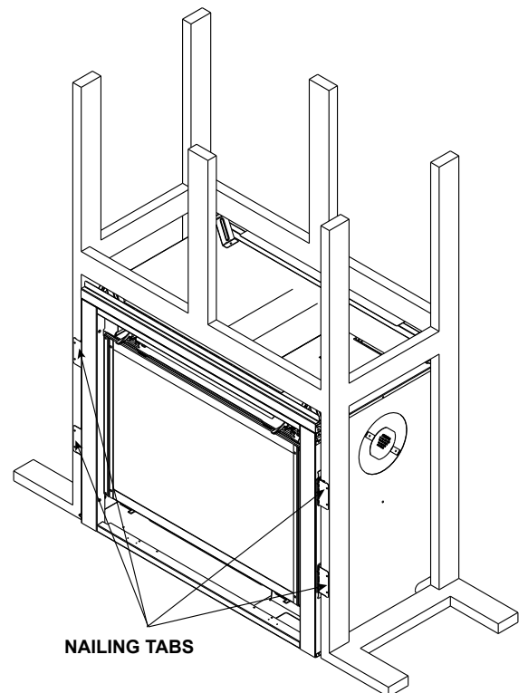
Figure 6.11 Securing An Appliance
