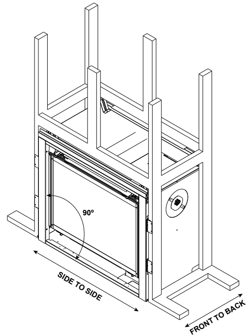
Figure 6.10 Proper Positioning and Leveling of an Appliance
