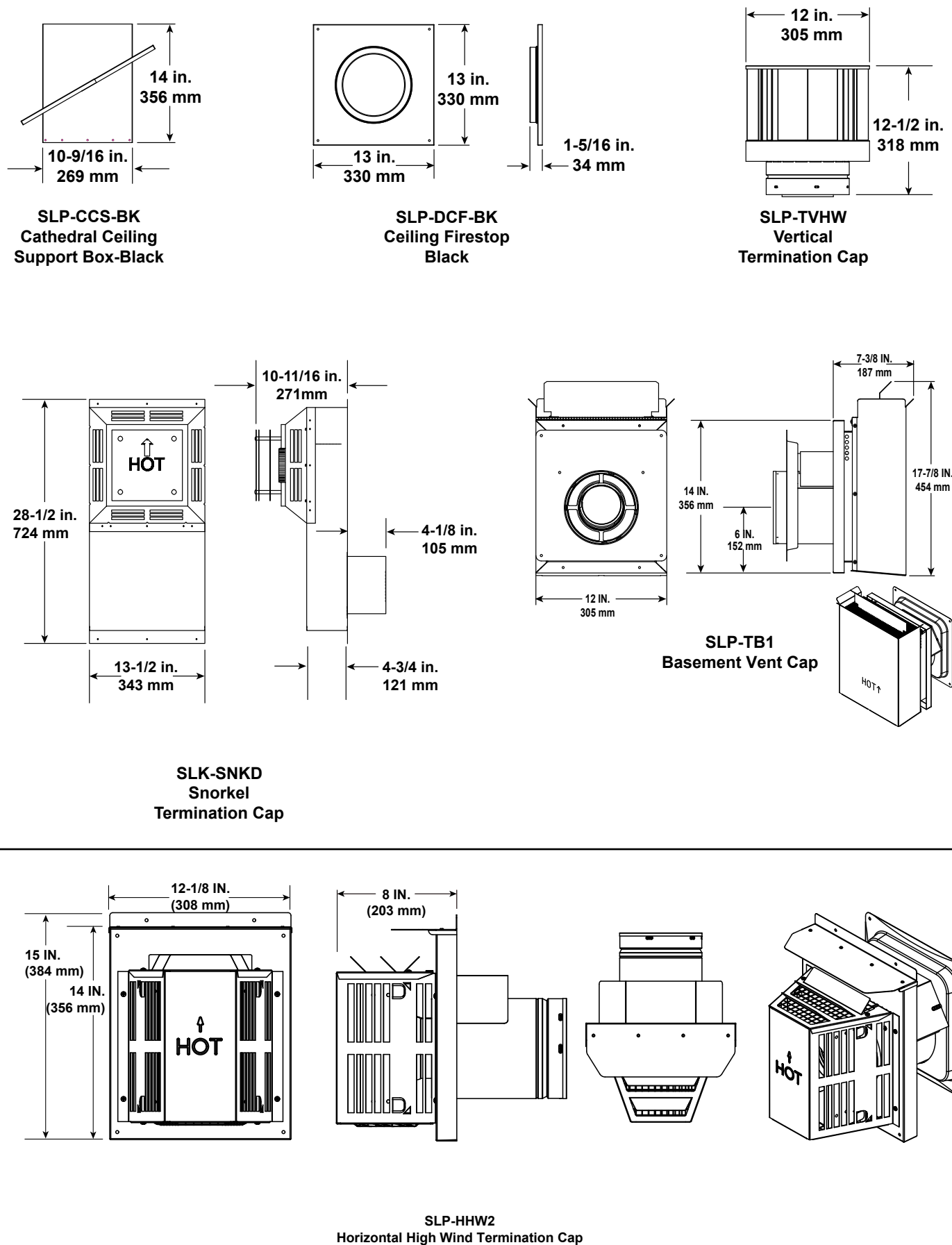
Figure 12.10 SLP Series Vent Components
