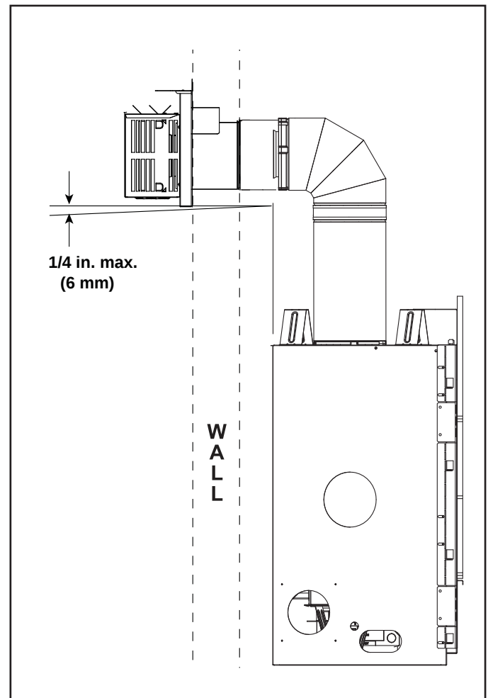
Figure 4.11 Vent Cap
