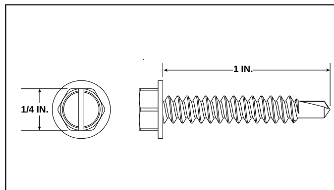
Figure 9.6 One Inch Mixing Screw
