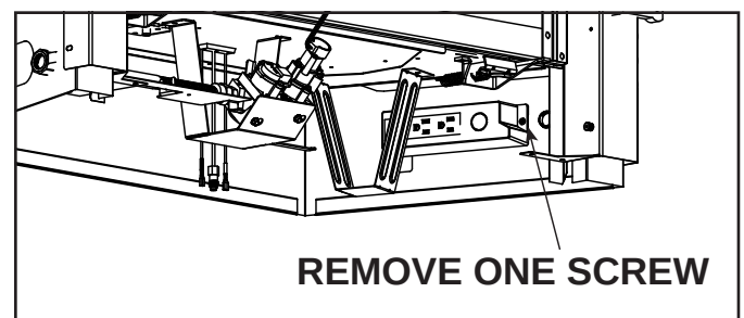
Figure 8.3 Junction Box Detail - COSMO32-IFT-B
