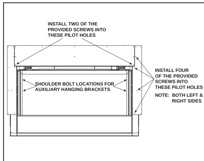
Figure 6.8 Installation of the Side Non-Combustible Components
