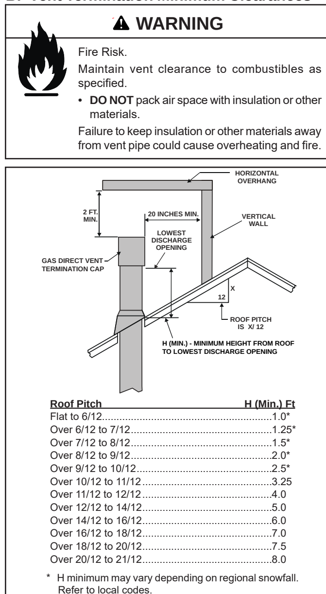
Figure 4.1 Minimum Height From Roof to Lowest Discharge Opening
