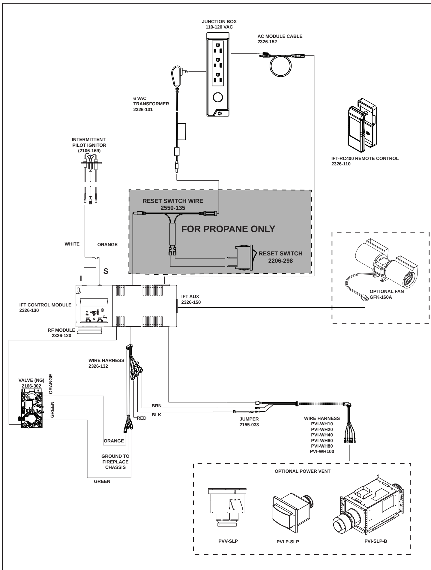
Figure 8.7 Intellifire Touch Wiring Diagram with Power Vent Diagram
