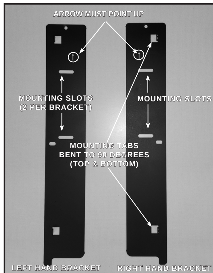
Figure 6.9 Auxiliary Hanging Brackets - Bent For Installation
