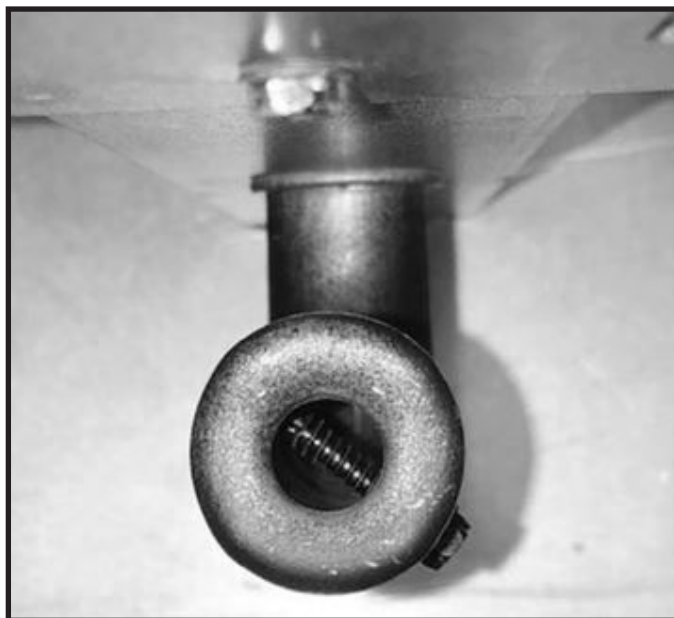
Figure 9.7 Mixing Screw Installed
