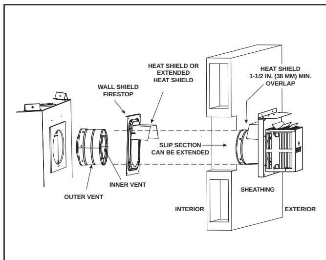
Figure 7.12 Venting Through the Wall
