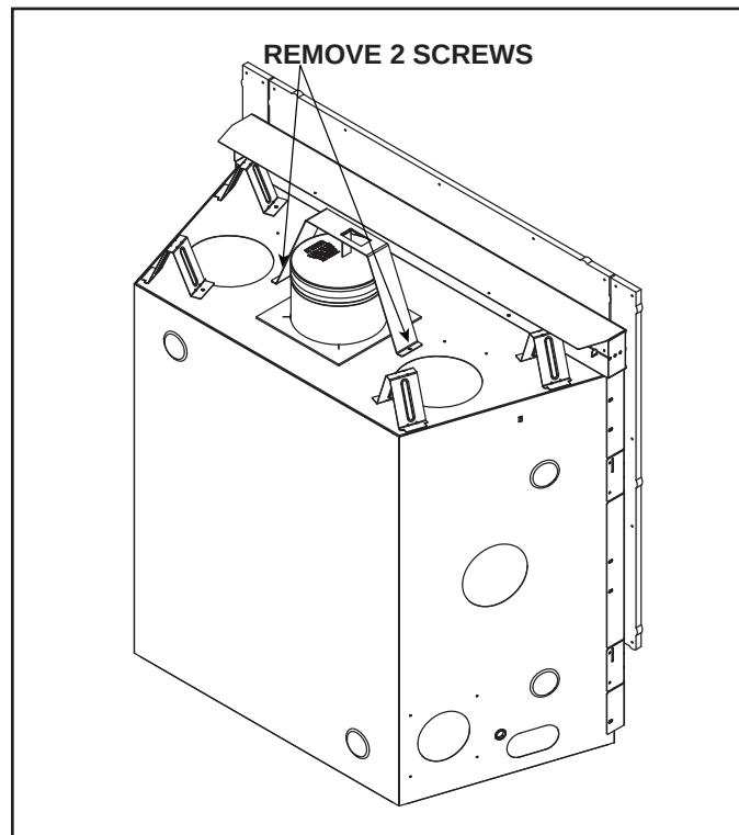
Figure 6.3 COSMO32-IFT-B - Shipping Support in Shipping Position
