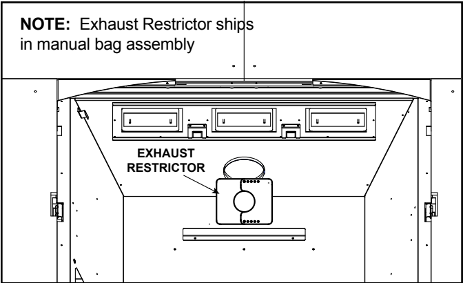
Figure 4.13 Exhaust Restrictor Installation
