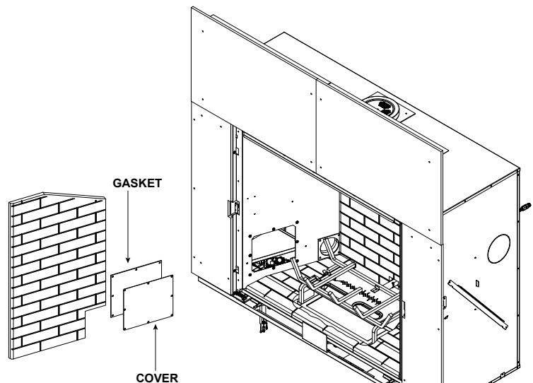
ACCESS THROUGH FIREBOX (After installation of non-combustible board)
