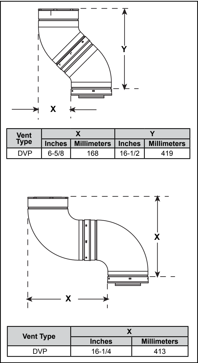
Figure 4.6 Vertical and Horizontal Offset for DVP Elbows
