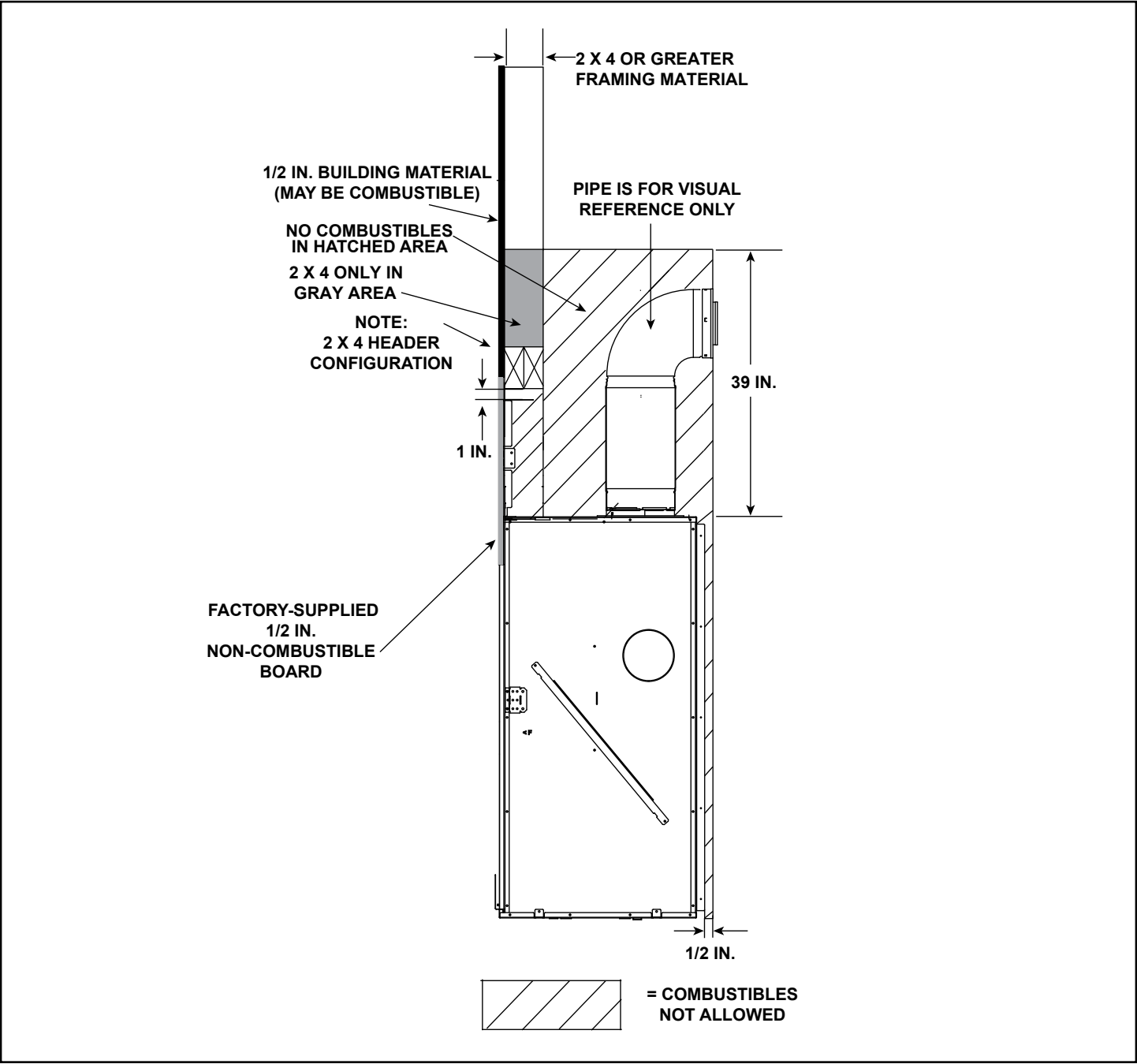
Figure 3.5 Non-Combustible Zone
