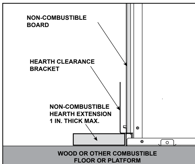
Figure 3.9 Appliance Installed on Combustible Surface Non-Combustible Hearth Extension REQUIRED.
