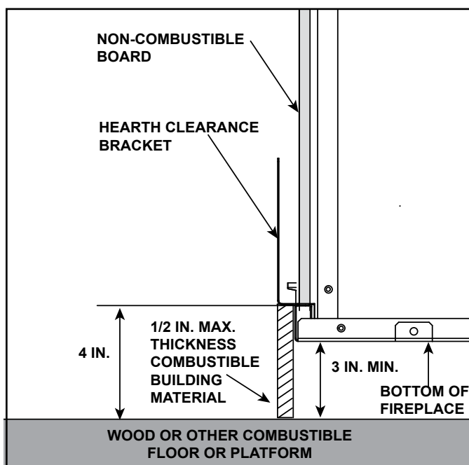
Figure 3.10 Appliance Raised a Minimum of 3 Inches Above Combustible Surface. Non-Combustible Hearth Extension NOT REQUIRED.
