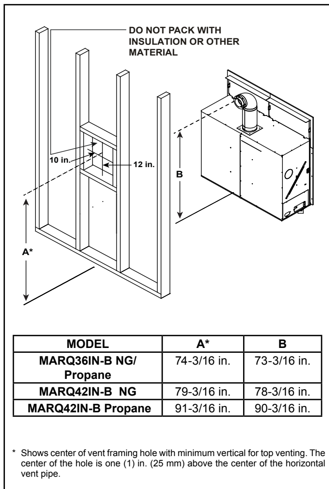
Figure 5.2 Wall Penetration
