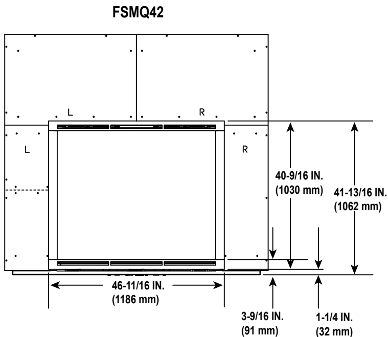
Figure 3.3 Decorative Barrier Front Dimensions
