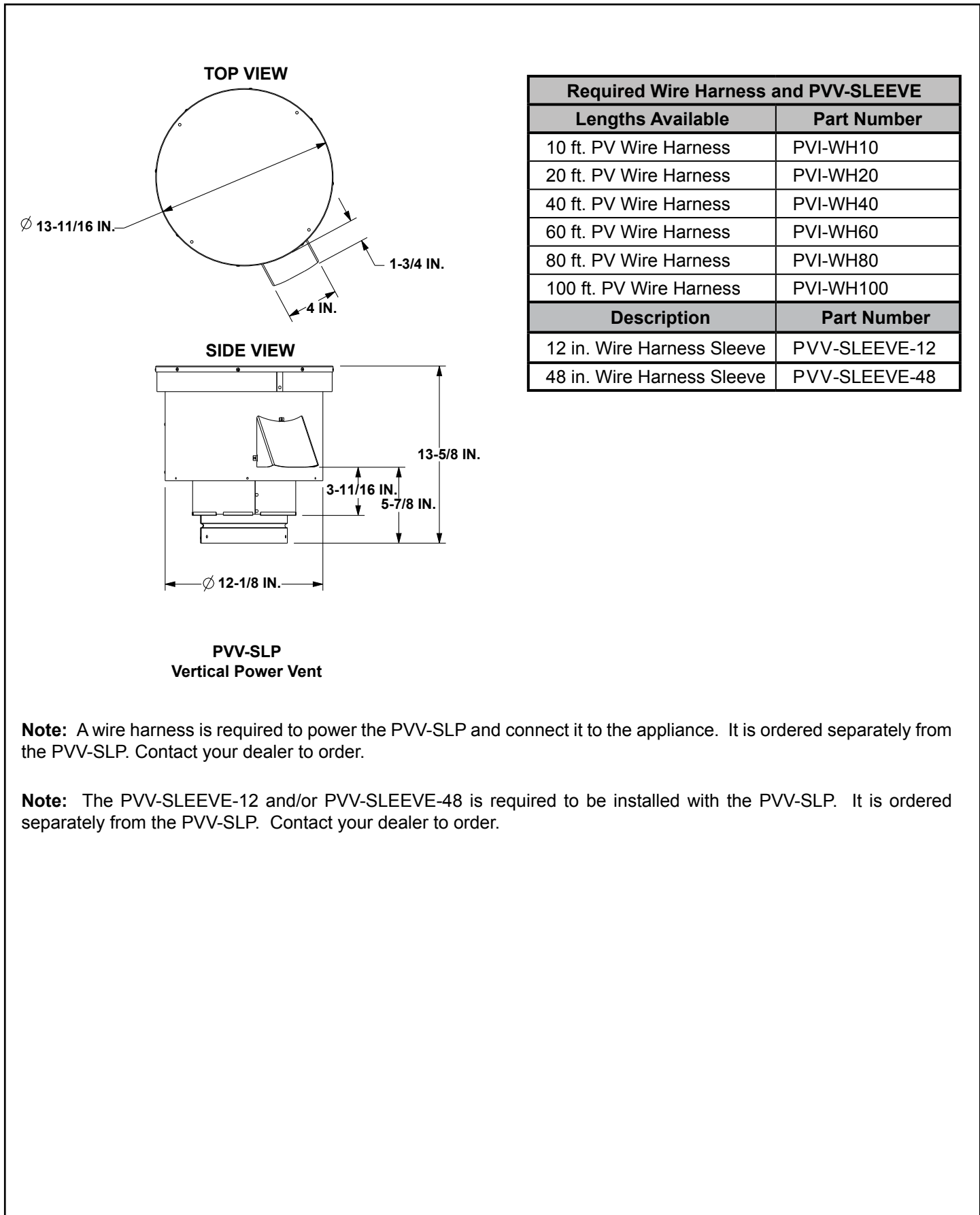
Figure 12.4 PVV-SLP Vent Components
