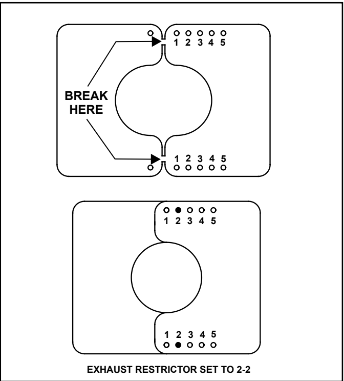
Figure 4.14 Exhaust Restrictor Installation
