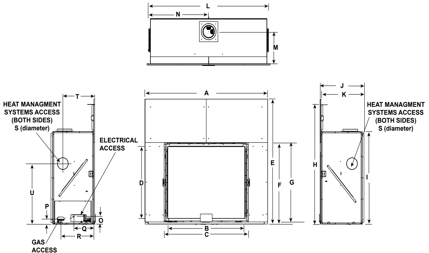
Appliance Dimensions Table MARQ36IN-B
