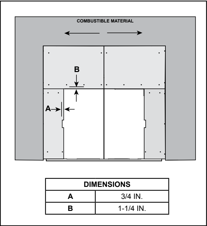
Figure 10.11 Inside Fit Decorative Barrier Fronts
