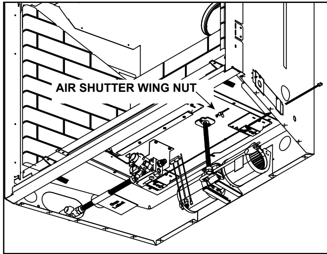
Figure 9.2 Air Shutter (Generic Fireplace Shown)
