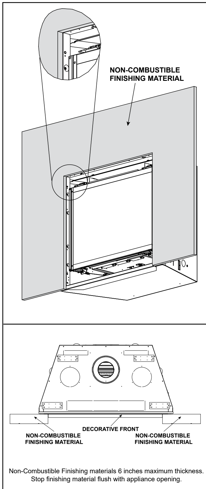
Figure 10.15 Inside Fit Method
