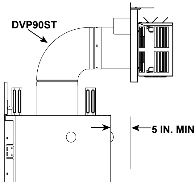
Figure 3.11 DVP-TRAP1 Exception (2 x 4 Construction)
