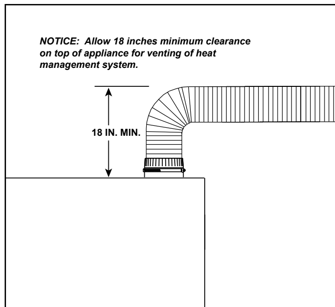
Figure 3.8 Clearance for Heat Management System
