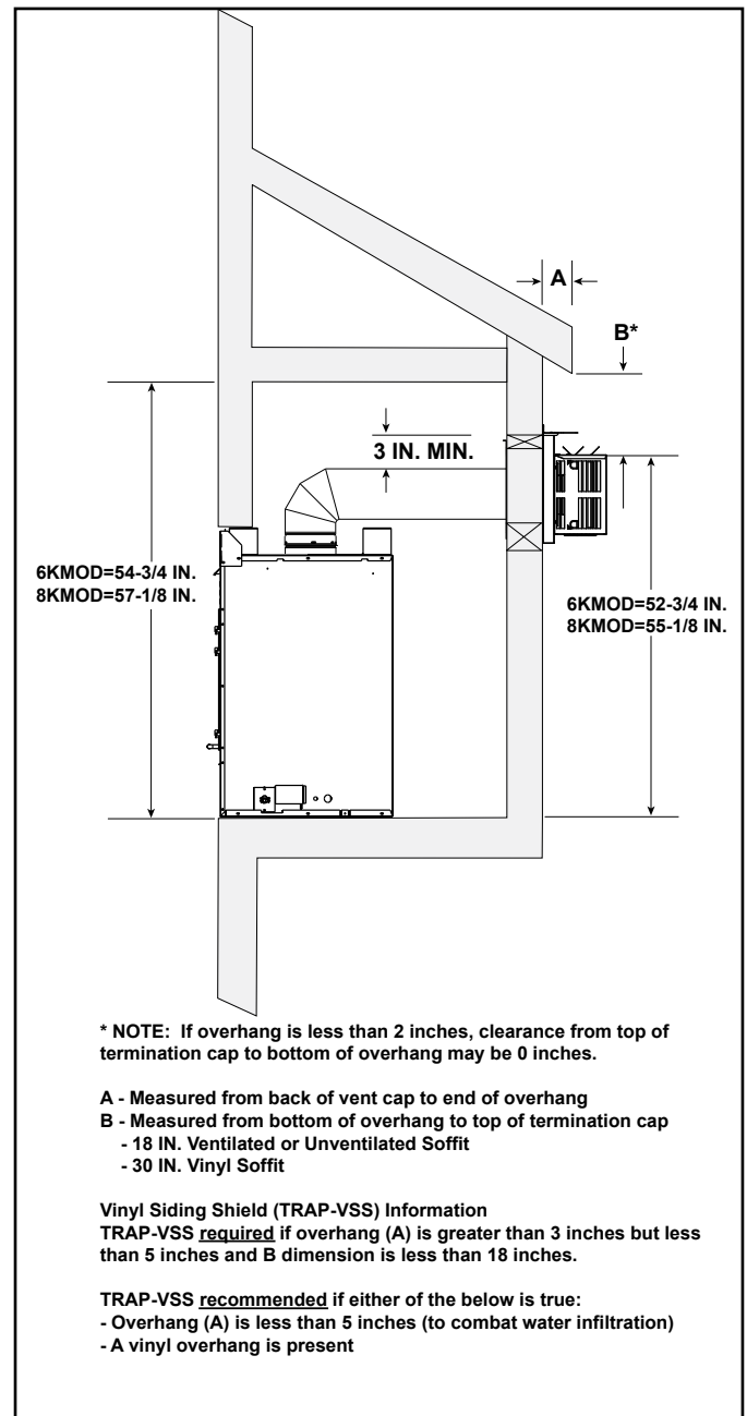
Figure 3.16 Exterior Chase - Minimum Height Requirements
