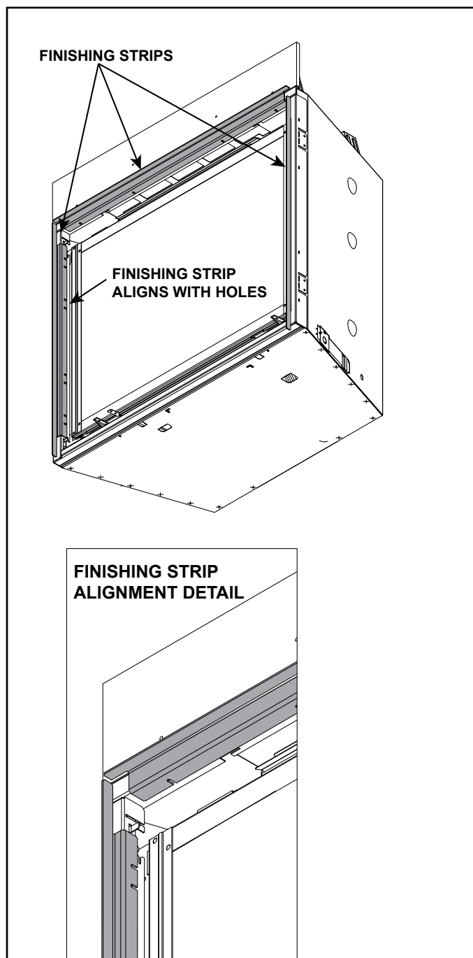
Figure 10.17 Install Finishing Strips
