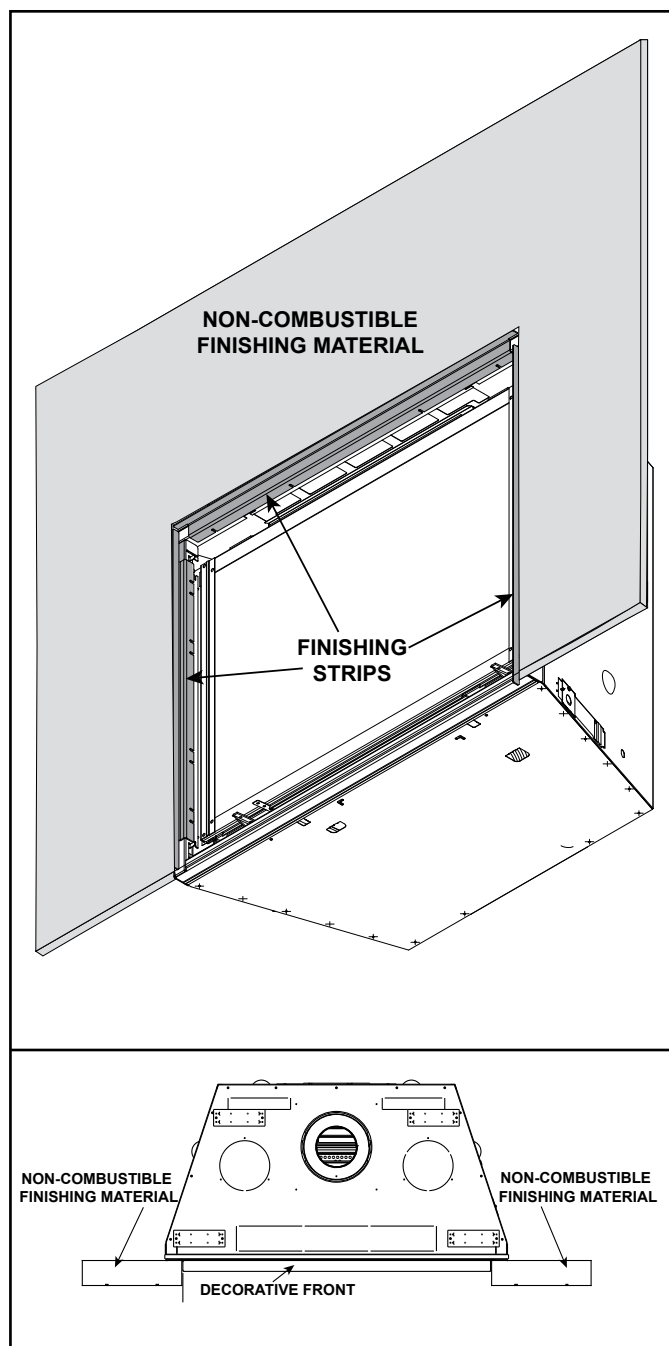
Figure 10.16 Non-Combustible Finishing Material Thickness Greater Than One Inch - Finishing Strips Required
