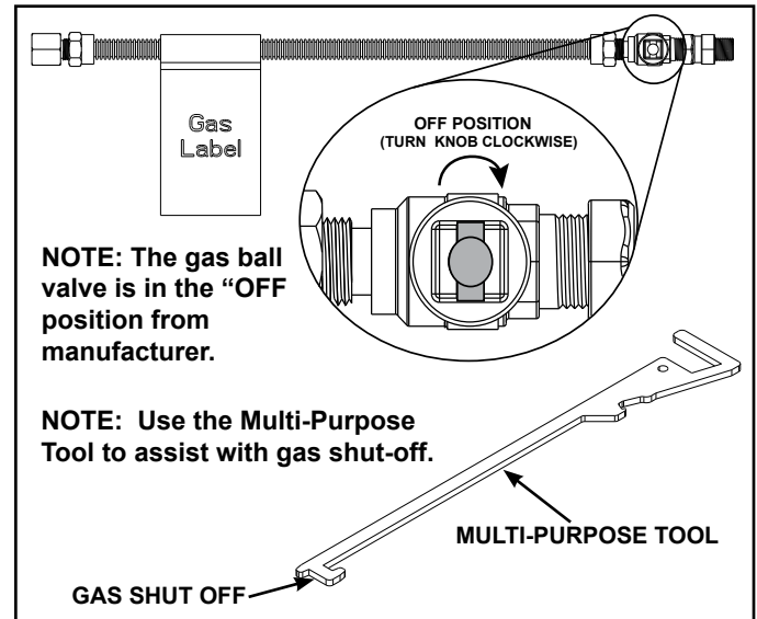
Figure 7.1 Gas Shut-off
