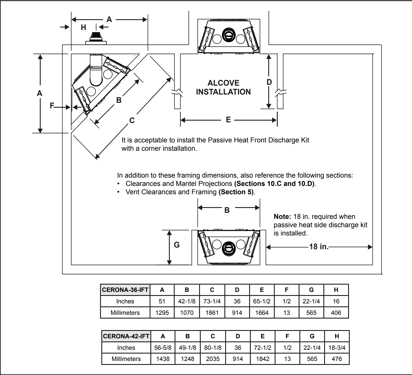
Figure 3.3 Appliance Locations
