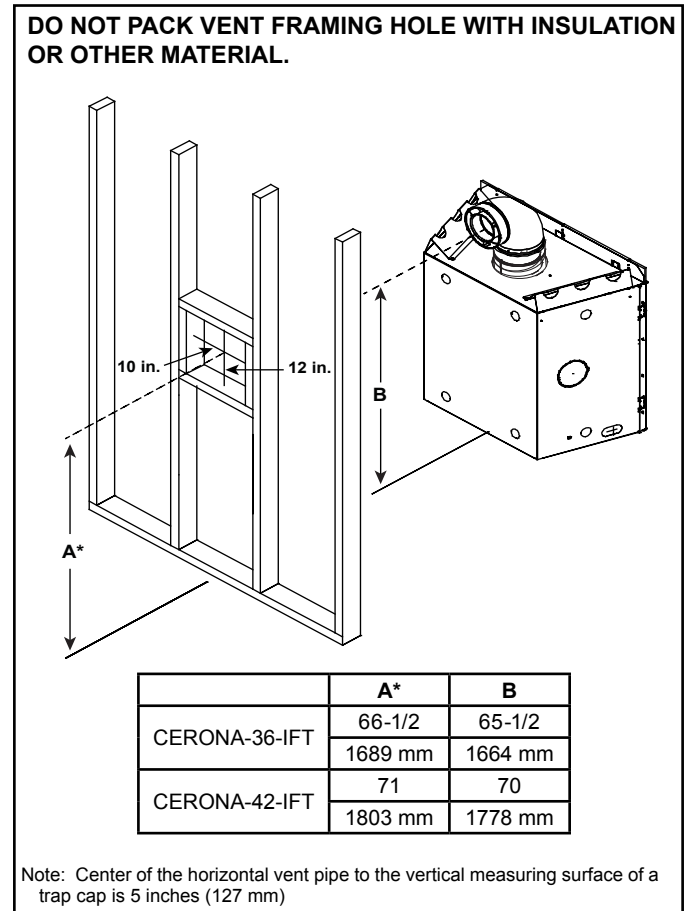
Figure 5.2 Wall Penetration
