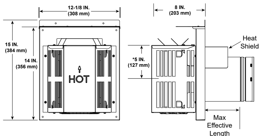
SLP-TRAP Horizontal Termination Cap
