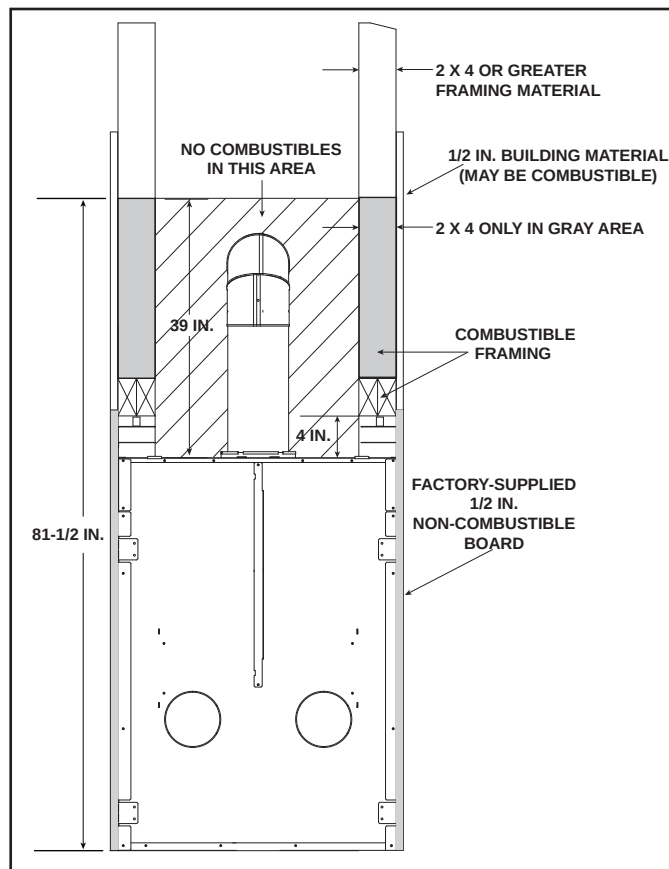
Figure 3.7 Non-Combustible Zone
