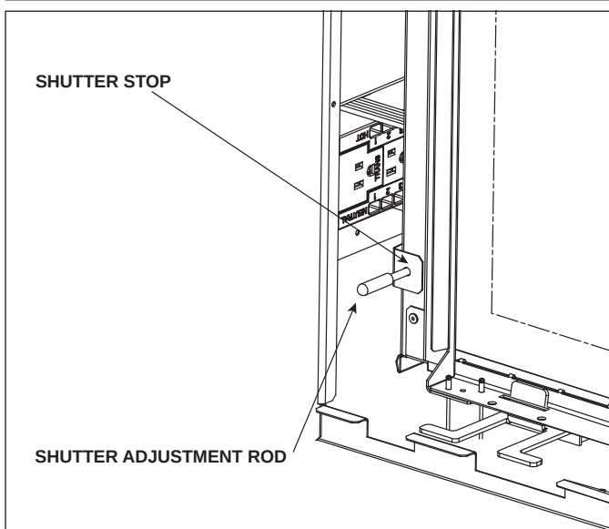
Figure 9.1 Shutter Adjustment Rod and Shutter Stop
