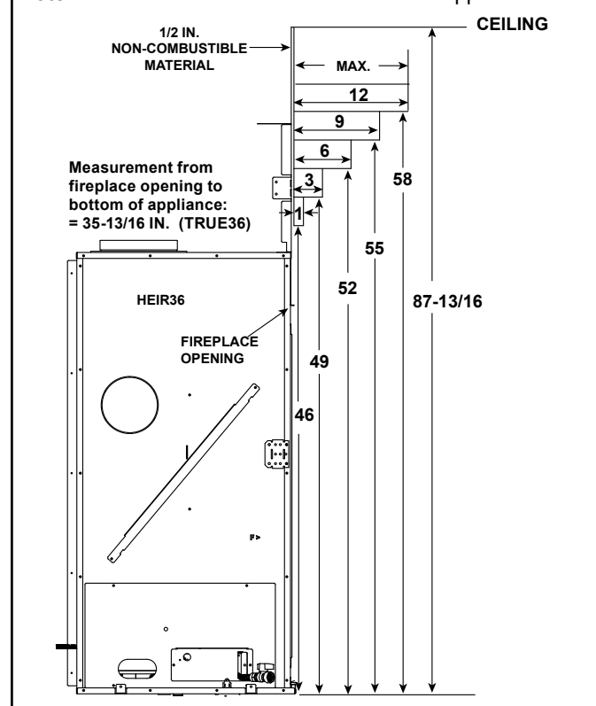
Figure 10.9 Combustible Mantel Allowance - TRUE-36
