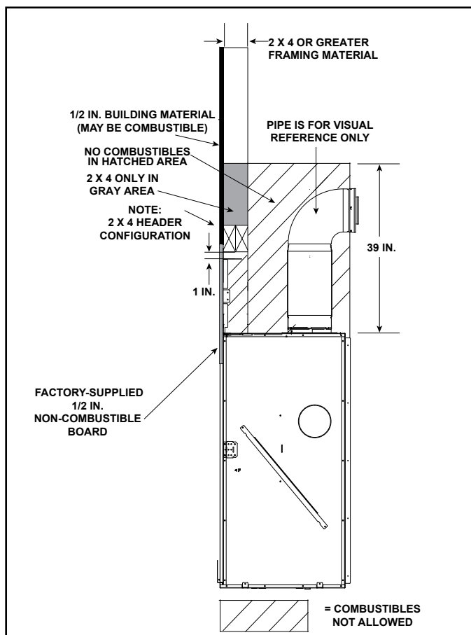
Figure 10.8 Non-Combustible Zone
