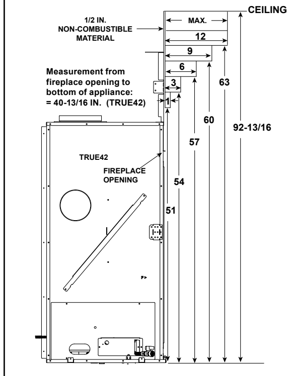
Figure 10.10 Combustible Mantel Allowance - TRUE-42
