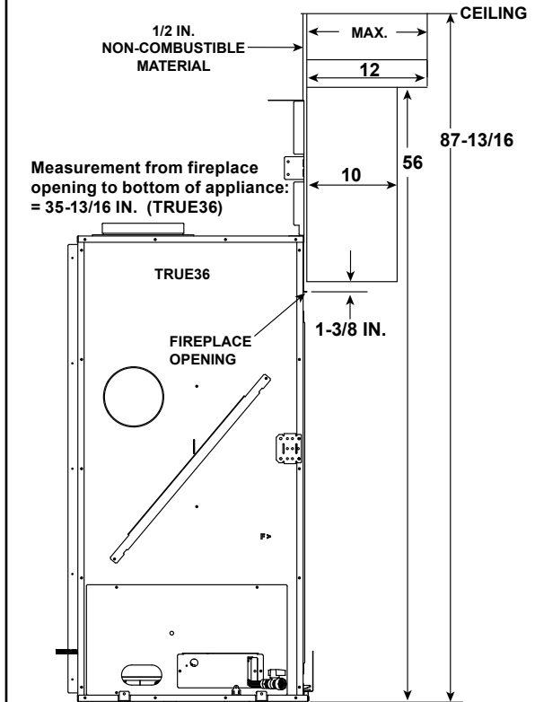
Figure 10.12 Non-Combustible Mantel Allowance - TRUE-36
