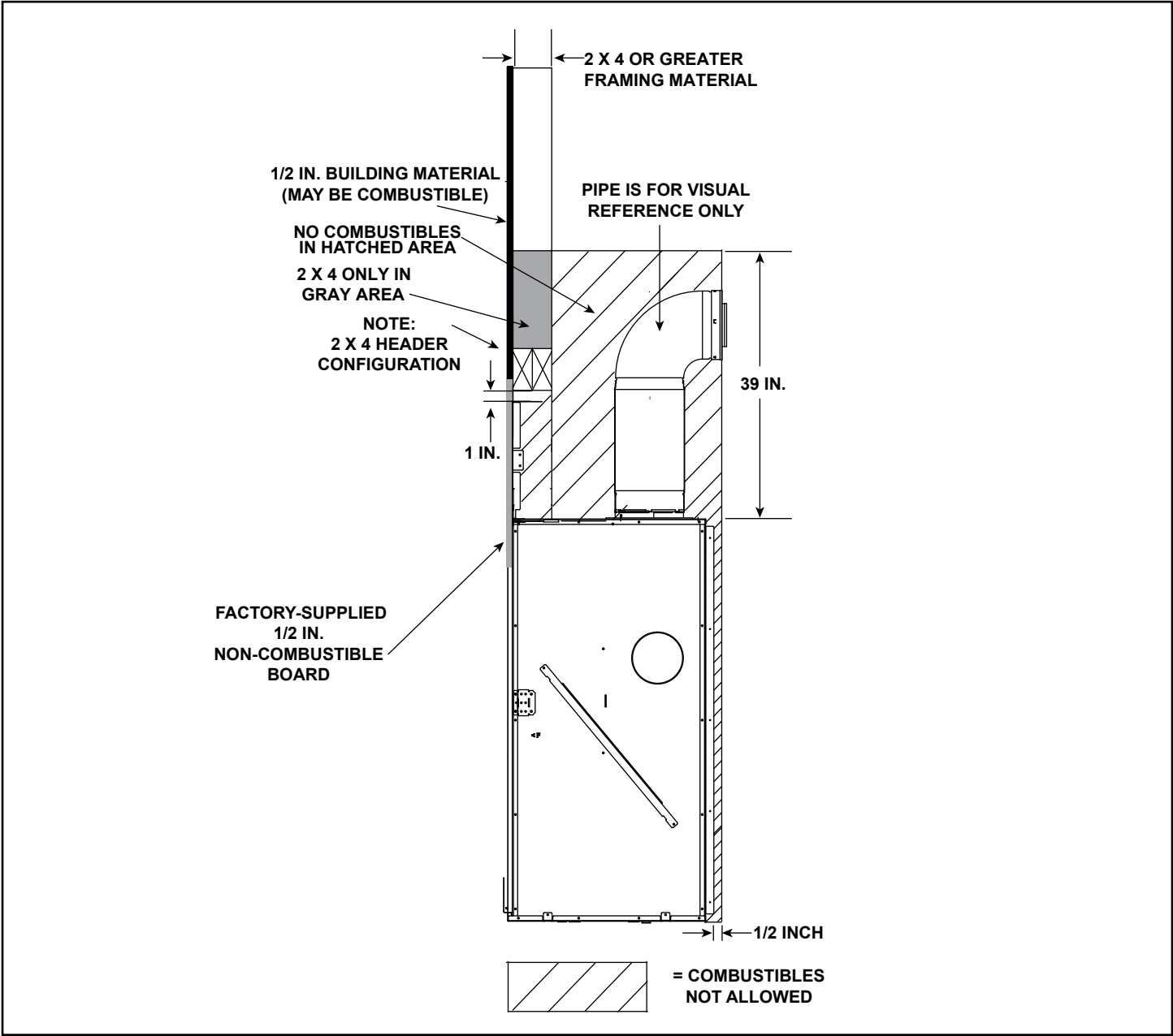
Figure 3.7 Non-Combustible Zone
