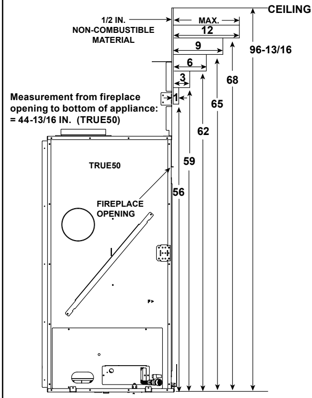
Figure 10.11 Combustible Mantel Allowance - TRUE-50
