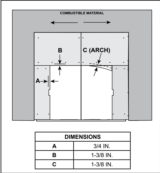
Figure 10.15 Inside Fit Decorative Fronts
