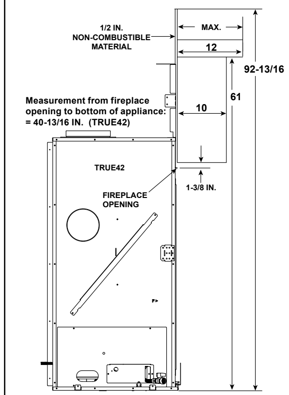
Figure 10.13 Non-Combustible Mantel Allowance - TRUE-42
