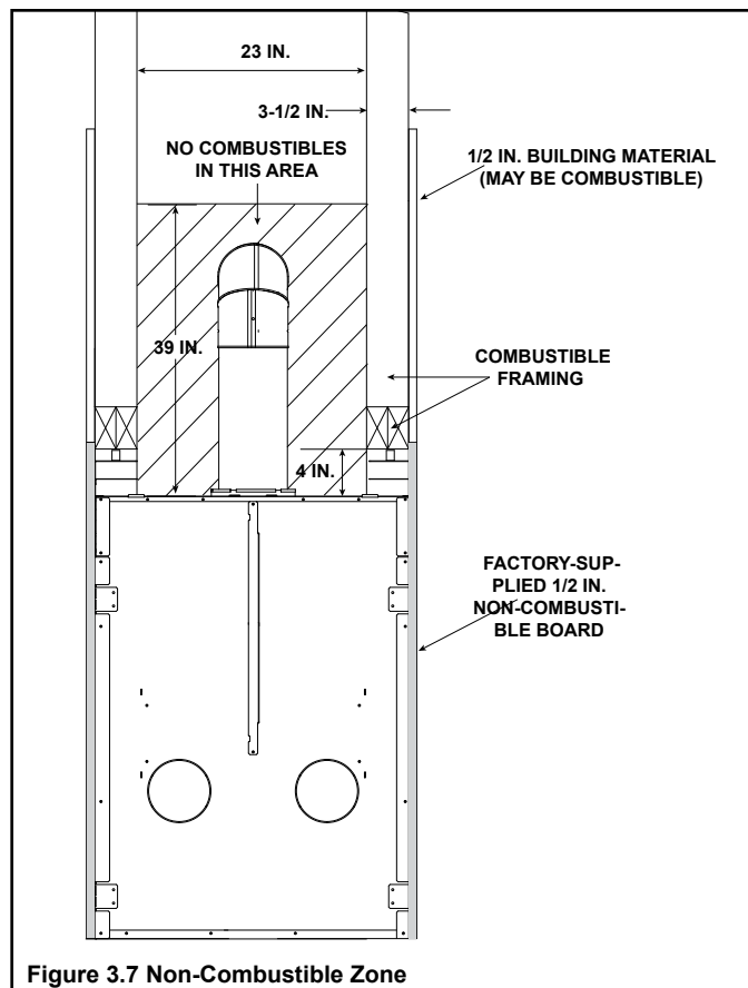
Figure 3.7 Non-Combustible Zone
