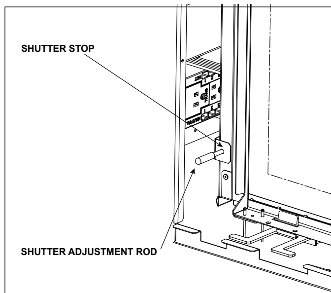
Figure 9.1 Shutter Adjustment Rod and Shutter Stop
