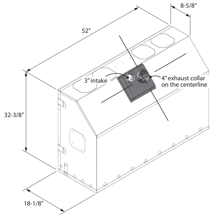
Dimensions with 1156CLA Co-Linear Adapter
