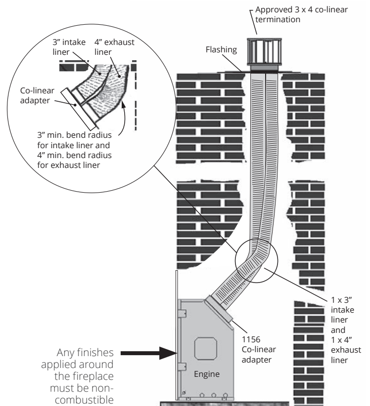
Co-Linear installation into existing fireplace
